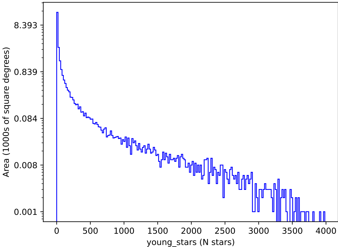
too_combined_no_nss_s10.0_v3.4_10yrs : young_stars
