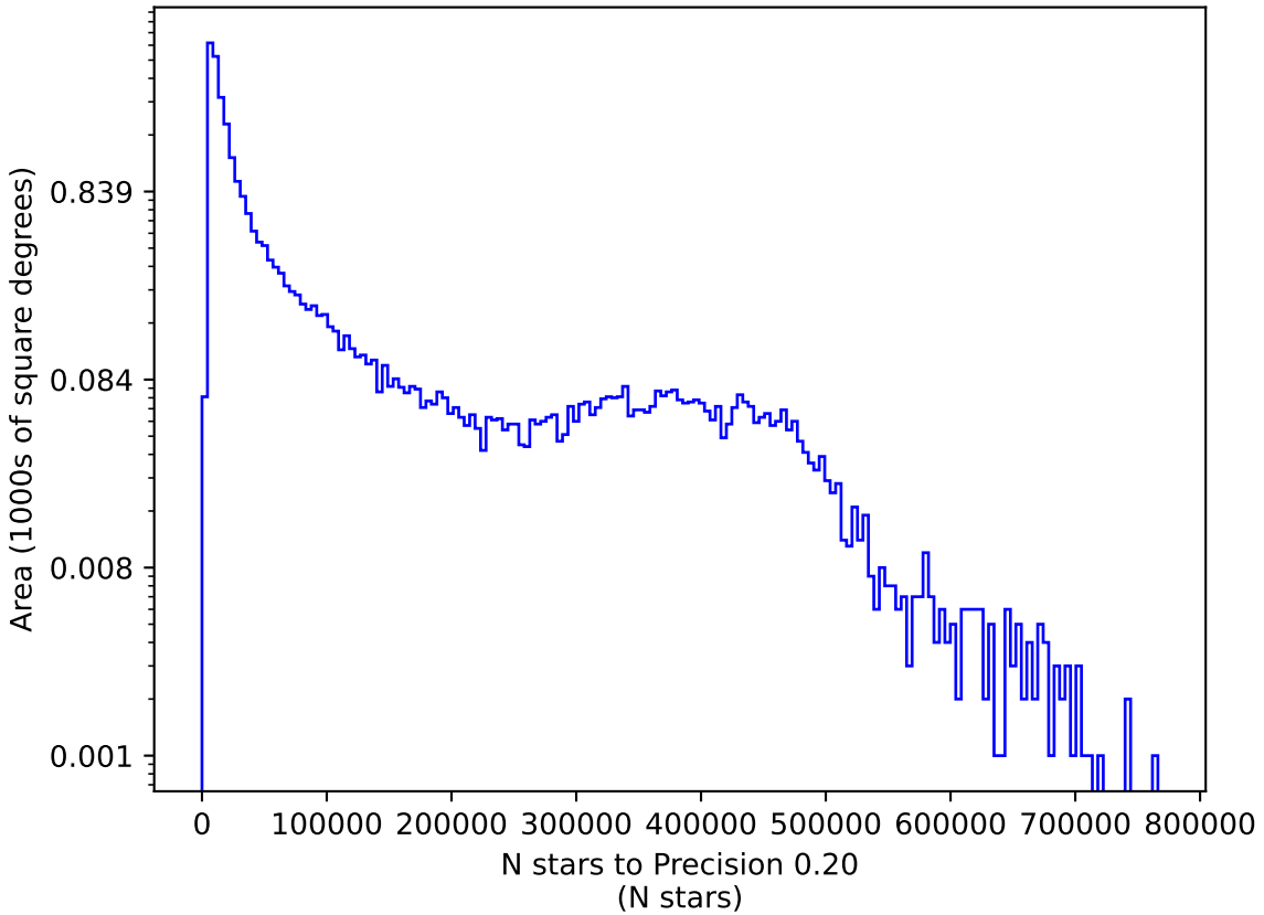
too_combined_no_nss_s10.0_v3.4_10yrs r: N stars to Precision 0.20
