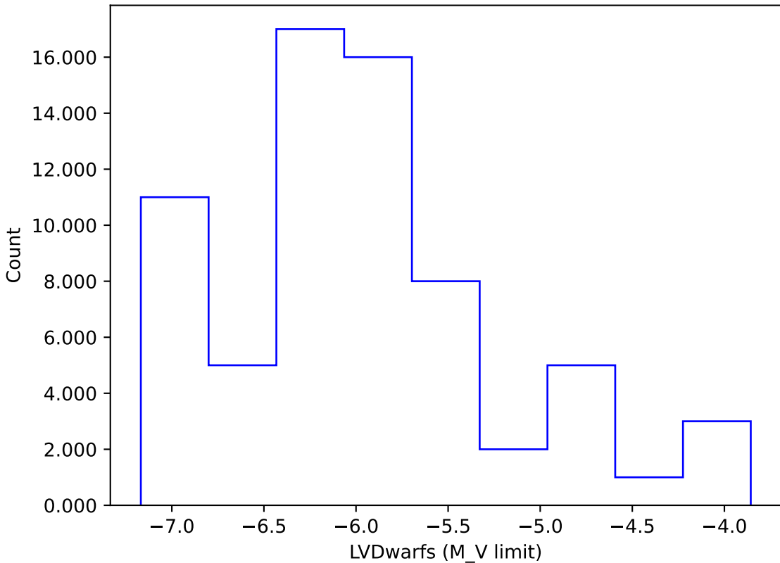
too_combined_no_nss_s10.0_v3.4_10yrs gi: LVDwarfs
