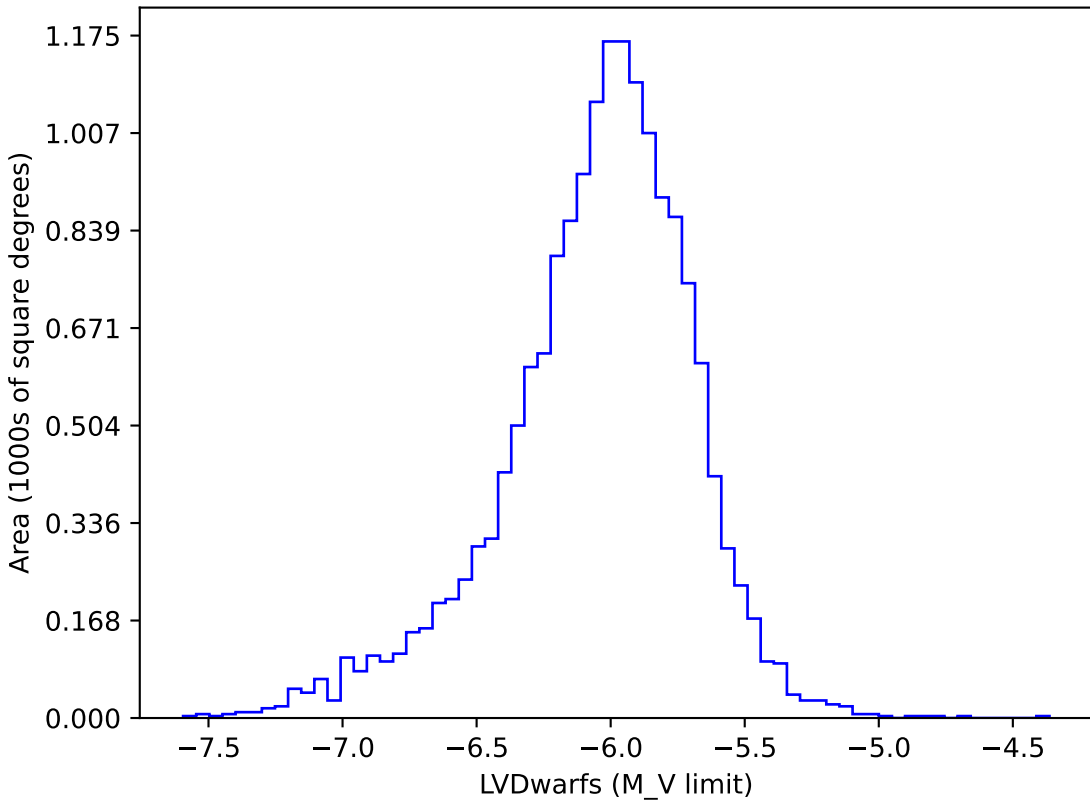
too_combined_no_nss_s10.0_v3.4_10yrs gi: LVDwarfs
