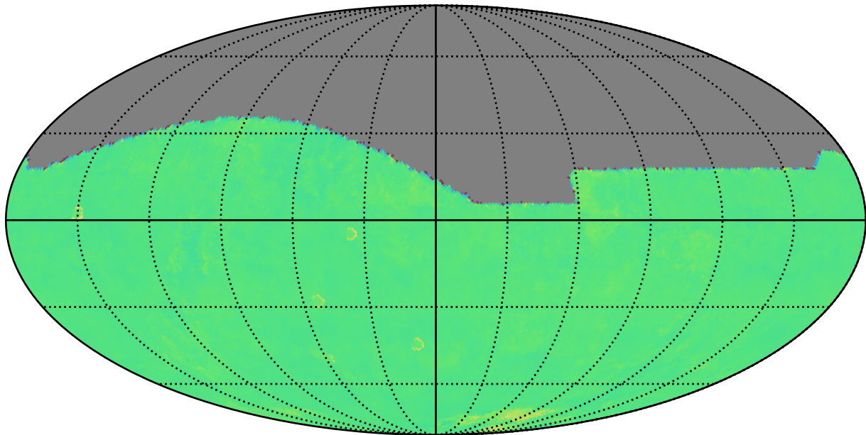
too_combined_no_nss_s10.0_v3.4_10yrs r: Kuiper rotTelPos
