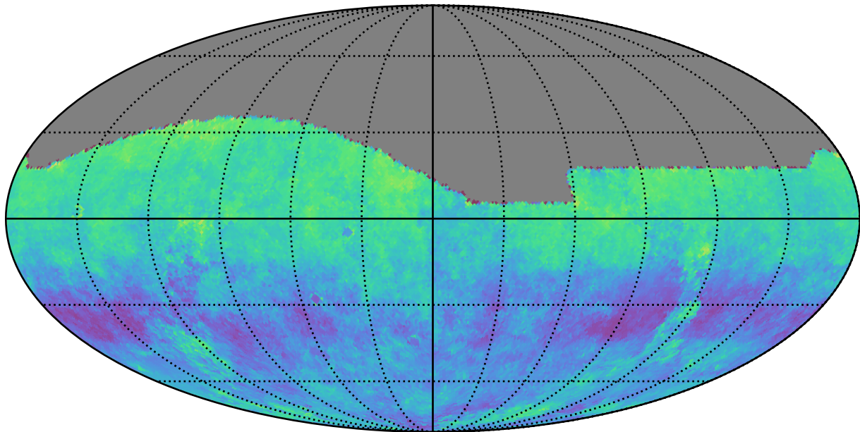
too_combined_no_nss_s10.0_v3.4_10yrs g: Kuiper rotSkyPos
