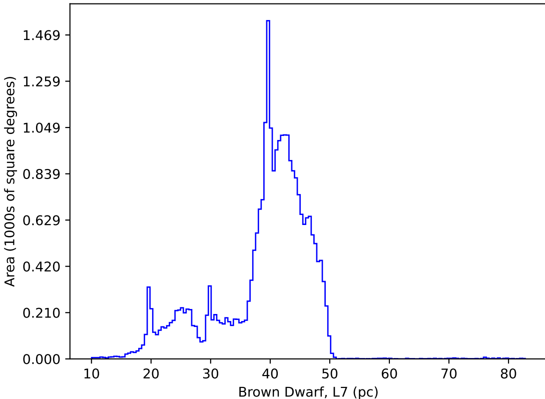
too_combined_no_nss_s10.0_v3.4_10yrs : Brown Dwarf, L7
