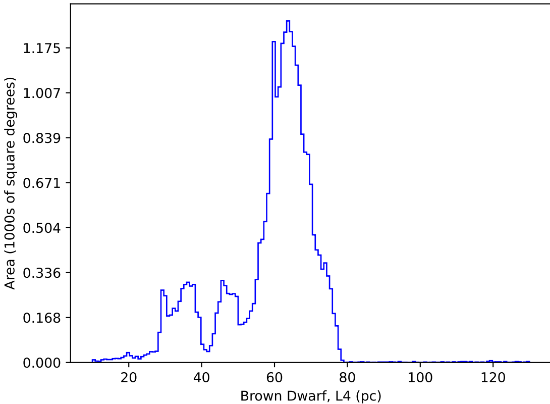
too_combined_no_nss_s10.0_v3.4_10yrs : Brown Dwarf, L4
