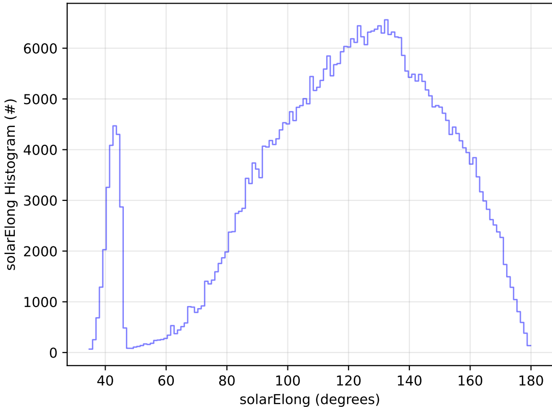
too_combined_no_nss_s10.0_v3.4_10yrs WFD z band: solarElong Histogram
