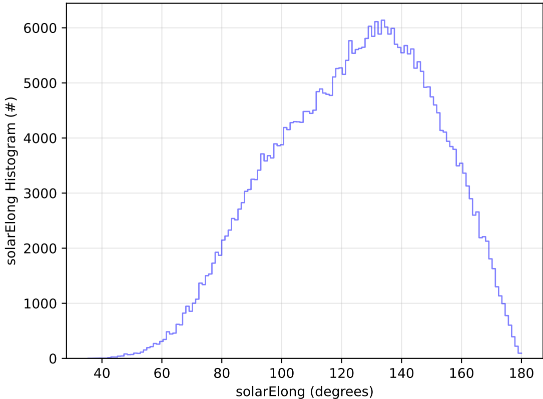
too_combined_no_nss_s10.0_v3.4_10yrs WFD y band: solarElong Histogram
