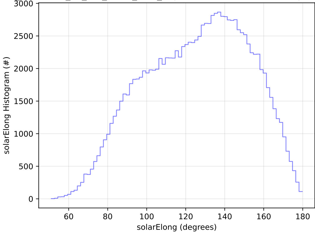
too_combined_no_nss_s10.0_v3.4_10yrs WFD u band: solarElong Histogram
