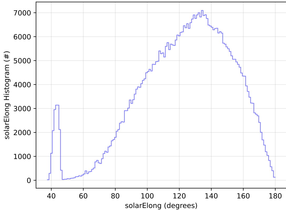
too_combined_no_nss_s10.0_v3.4_10yrs WFD r band: solarElong Histogram
