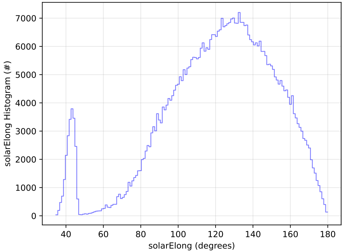
too_combined_no_nss_s10.0_v3.4_10yrs WFD i band: solarElong Histogram
