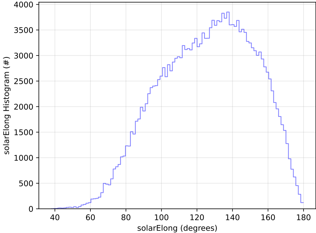
too_combined_no_nss_s10.0_v3.4_10yrs WFD g band: solarElong Histogram
