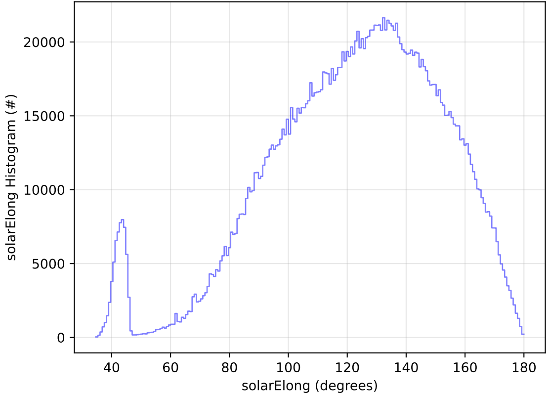
too_combined_no_nss_s10.0_v3.4_10yrs WFD all bands: solarElong Histogram
