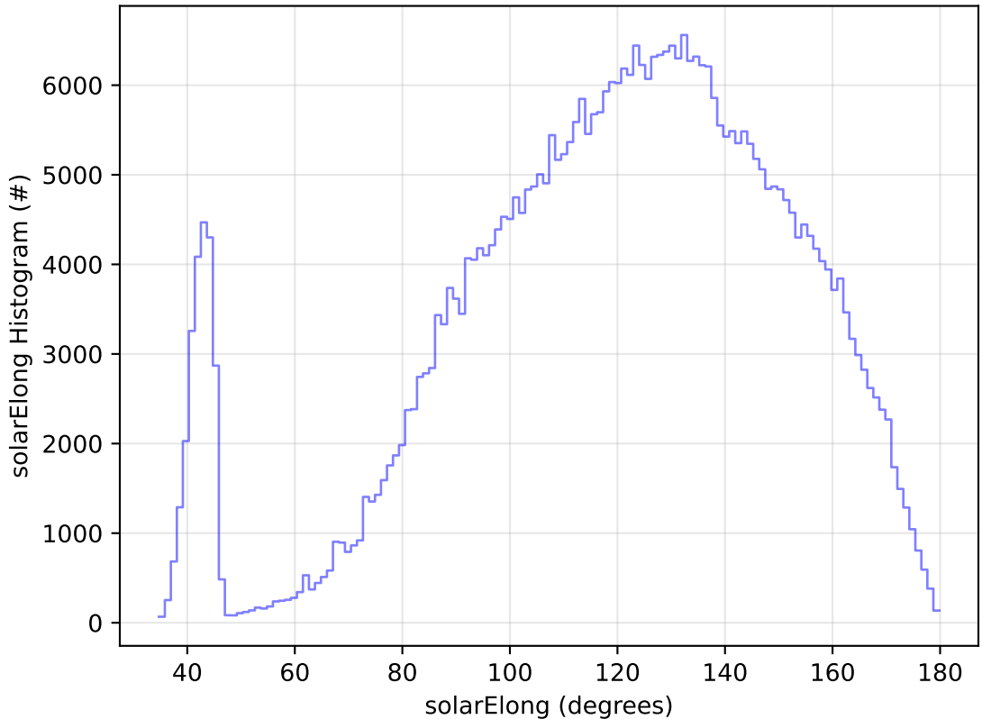
too_combined_no_nss_s10.0_v3.4_10yrs All sky z band: solarElong Histogram
