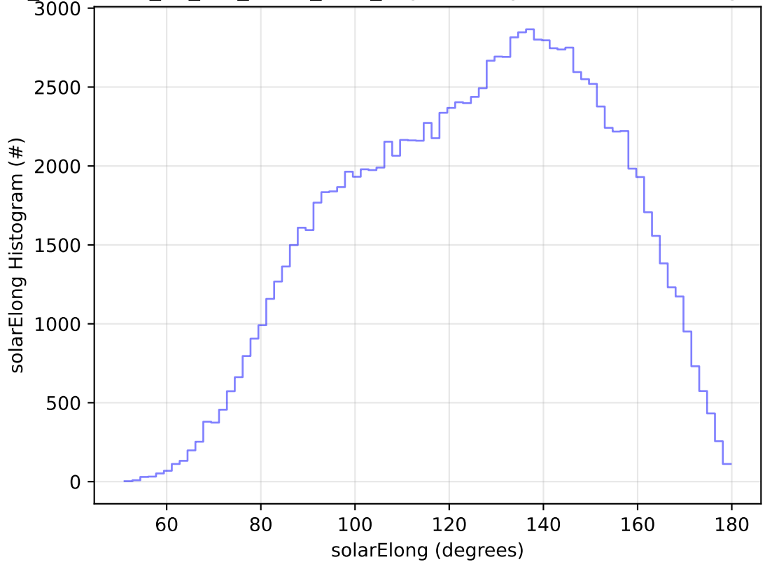
too_combined_no_nss_s10.0_v3.4_10yrs All sky u band: solarElong Histogram
