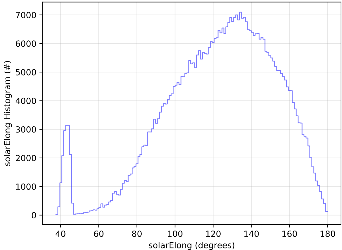
too_combined_no_nss_s10.0_v3.4_10yrs All sky r band: solarElong Histogram
