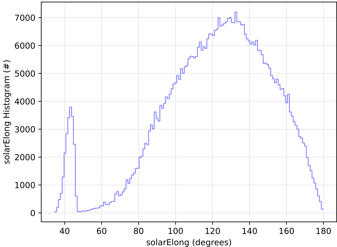
too_combined_no_nss_s10.0_v3.4_10yrs All sky i band: solarElong Histogram
