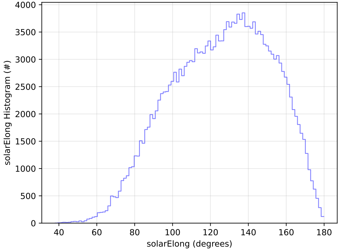
too_combined_no_nss_s10.0_v3.4_10yrs All sky g band: solarElong Histogram
