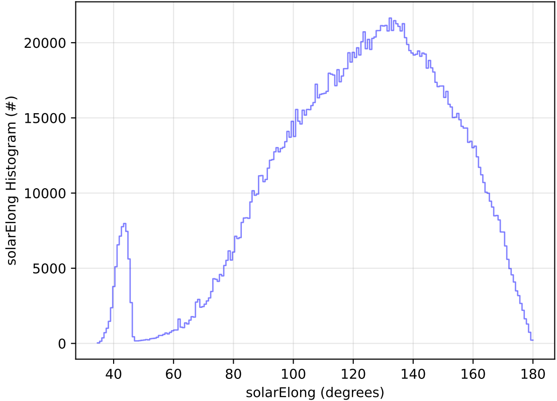
too_combined_no_nss_s10.0_v3.4_10yrs All sky all bands: solarElong Histogram
