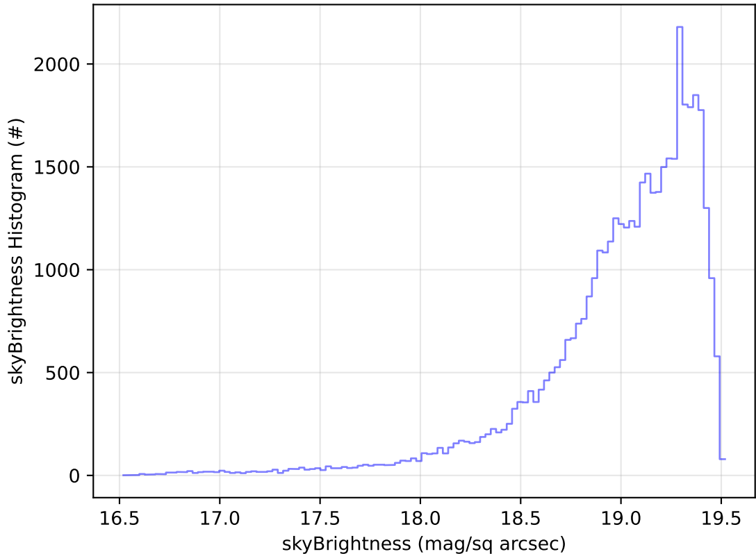
too_combined_no_nss_s10.0_v3.4_10yrs Yr 1 z band: skyBrightness Histogram
