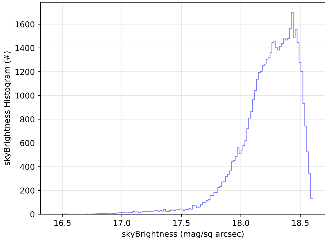
too_combined_no_nss_s10.0_v3.4_10yrs Yr 1 y band: skyBrightness Histogram
