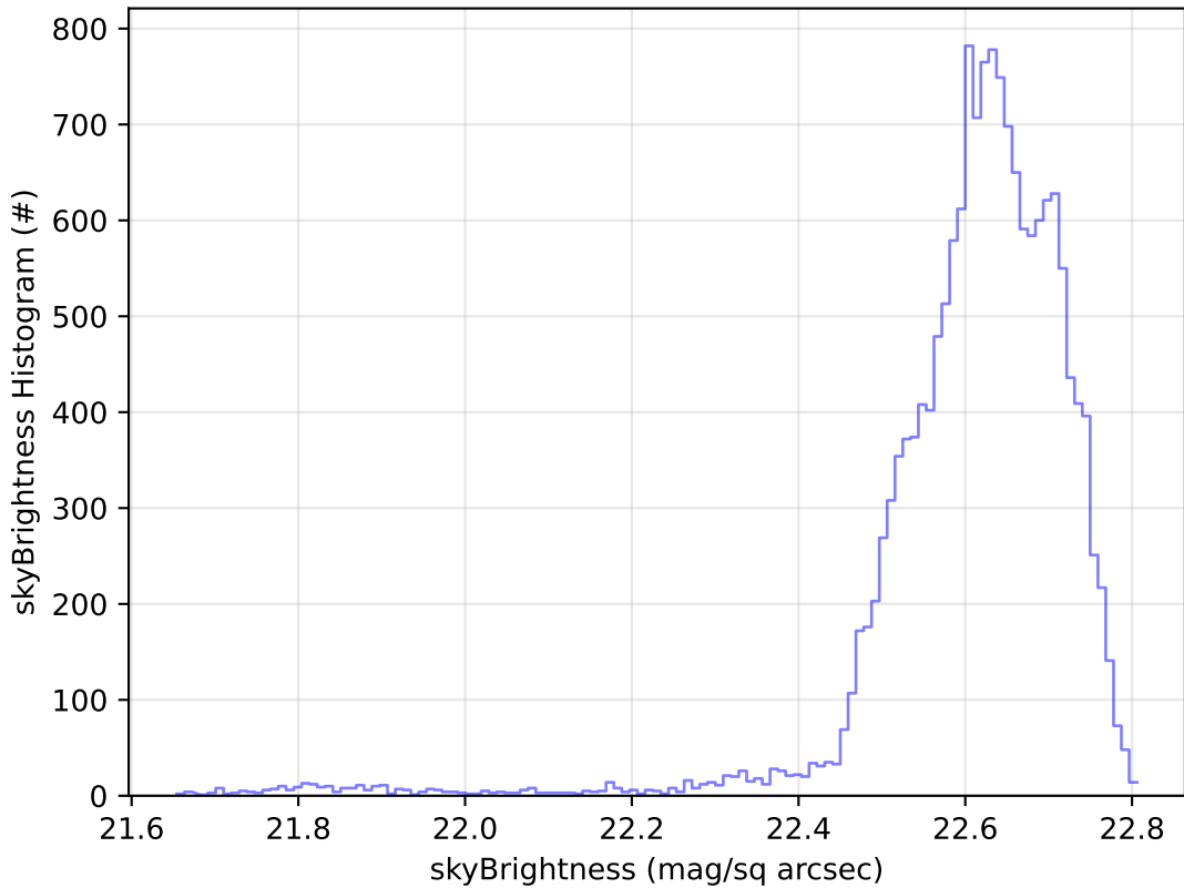
too_combined_no_nss_s10.0_v3.4_10yrs Yr 1 u band: skyBrightness Histogram
