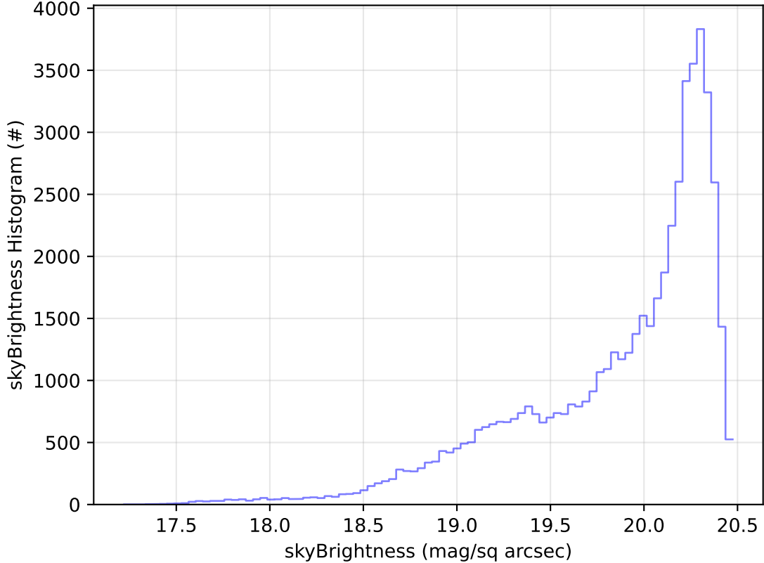
too_combined_no_nss_s10.0_v3.4_10yrs Yr 1 i band: skyBrightness Histogram
