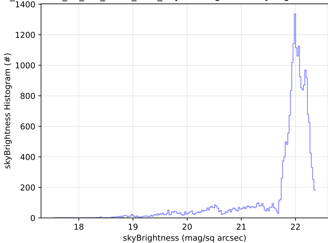
too_combined_no_nss_s10.0_v3.4_10yrs Yr 1 g band: skyBrightness Histogram
