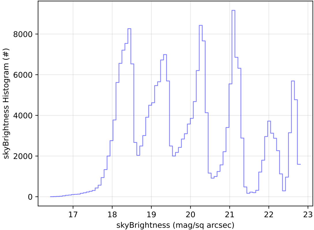
too_combined_no_nss_s10.0_v3.4_10yrs Yr 1 all bands: skyBrightness Histogram
