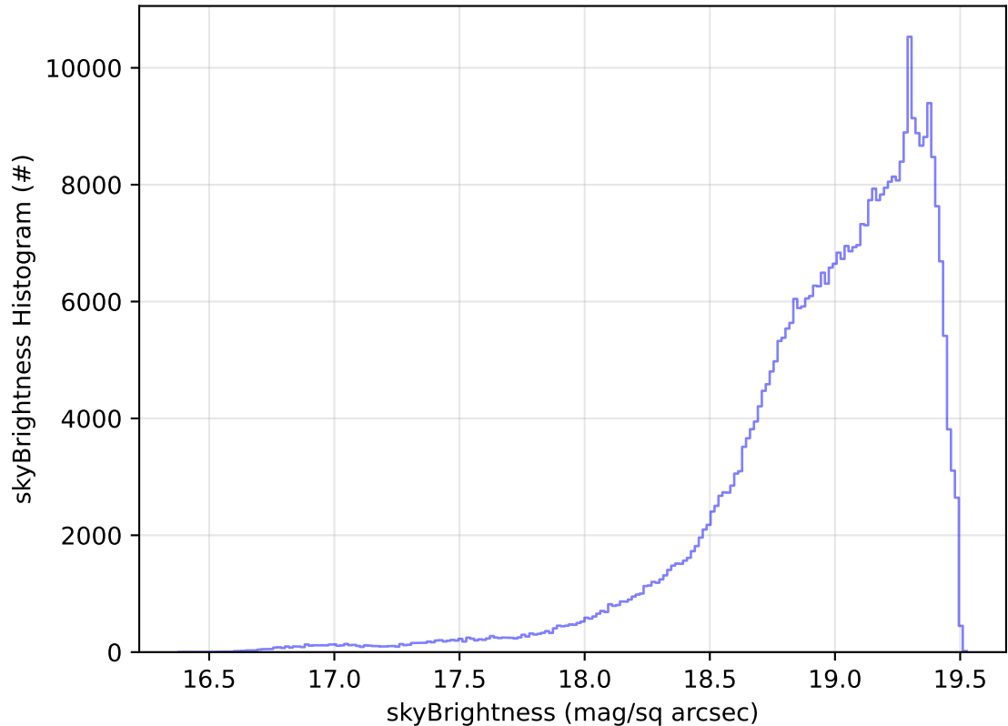
too_combined_no_nss_s10.0_v3.4_10yrs WFD z band: skyBrightness Histogram
