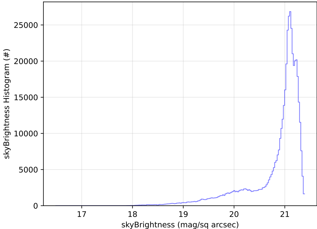
too_combined_no_nss_s10.0_v3.4_10yrs WFD r band: skyBrightness Histogram
