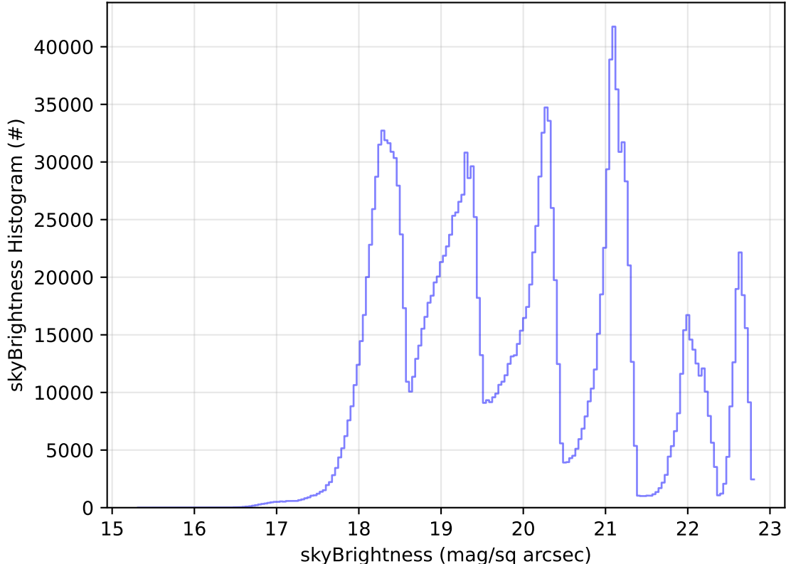
too_combined_no_nss_s10.0_v3.4_10yrs WFD all bands: skyBrightness Histogram
