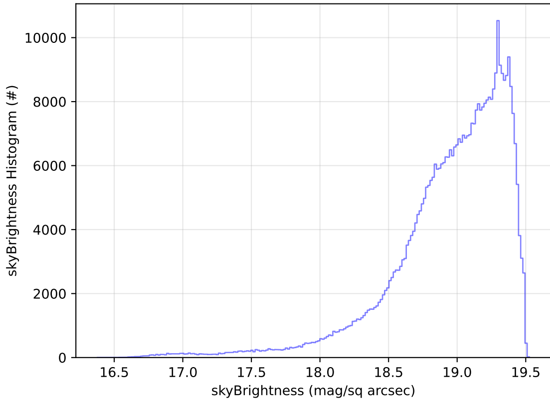
too_combined_no_nss_s10.0_v3.4_10yrs All sky z band: skyBrightness Histogram
