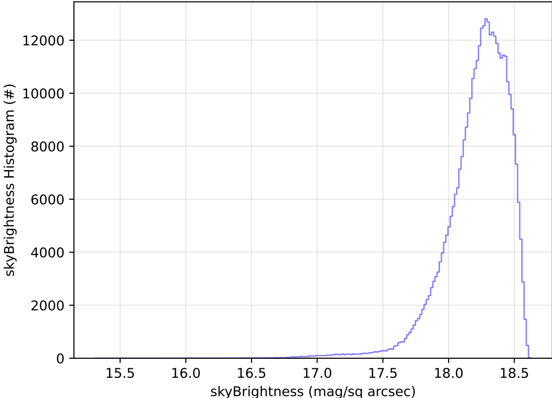
too_combined_no_nss_s10.0_v3.4_10yrs All sky y band: skyBrightness Histogram
