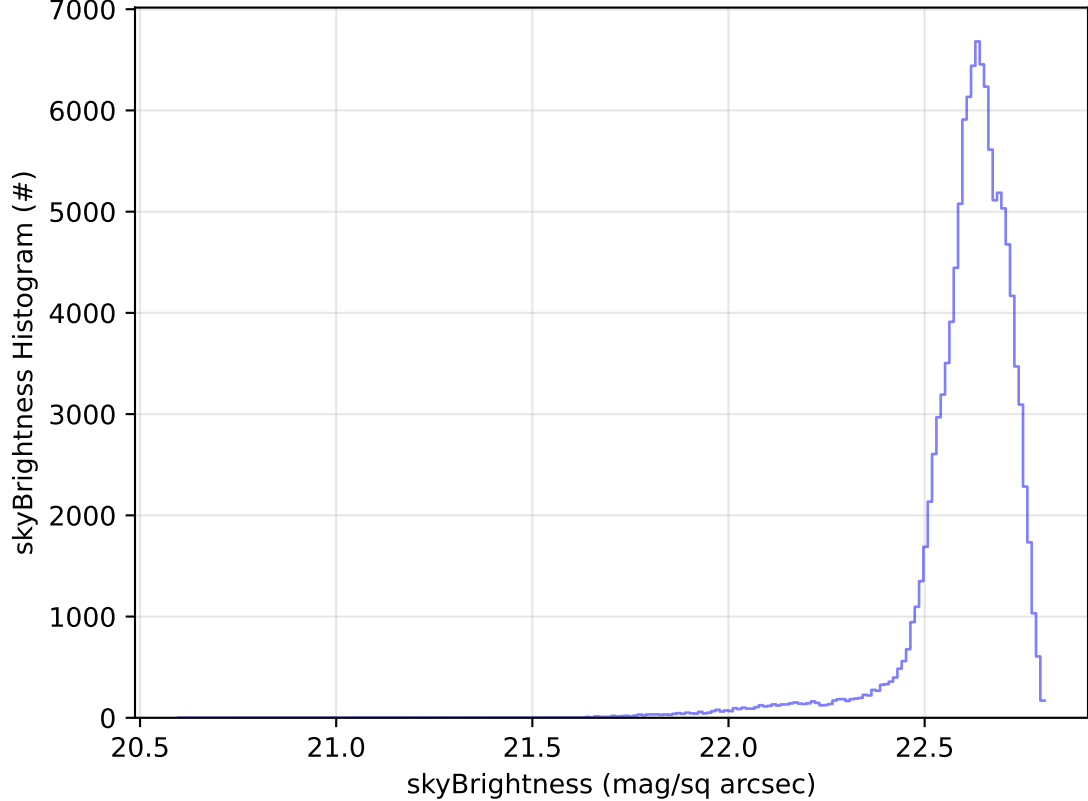
too_combined_no_nss_s10.0_v3.4_10yrs All sky u band: skyBrightness Histogram
