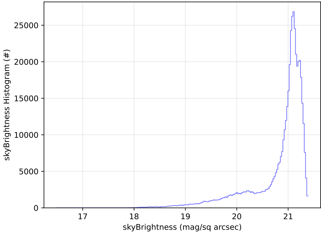
too_combined_no_nss_s10.0_v3.4_10yrs All sky r band: skyBrightness Histogram
