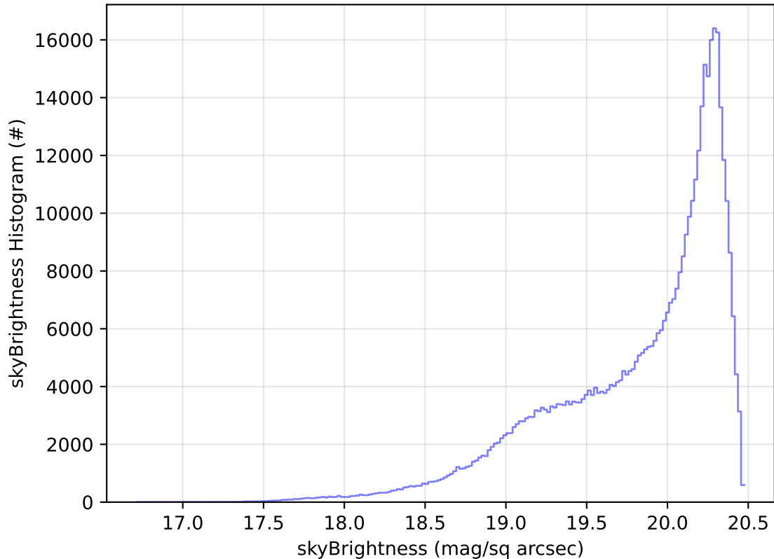
too_combined_no_nss_s10.0_v3.4_10yrs All sky i band: skyBrightness Histogram
