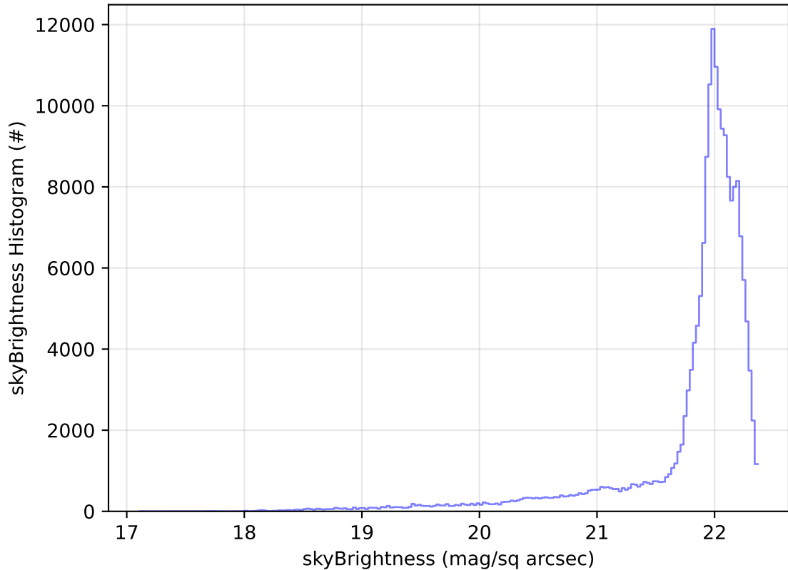
too_combined_no_nss_s10.0_v3.4_10yrs All sky g band: skyBrightness Histogram
