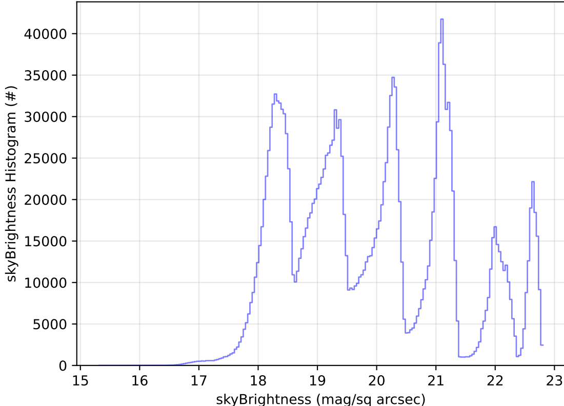
too_combined_no_nss_s10.0_v3.4_10yrs All sky all bands: skyBrightness Histogram
