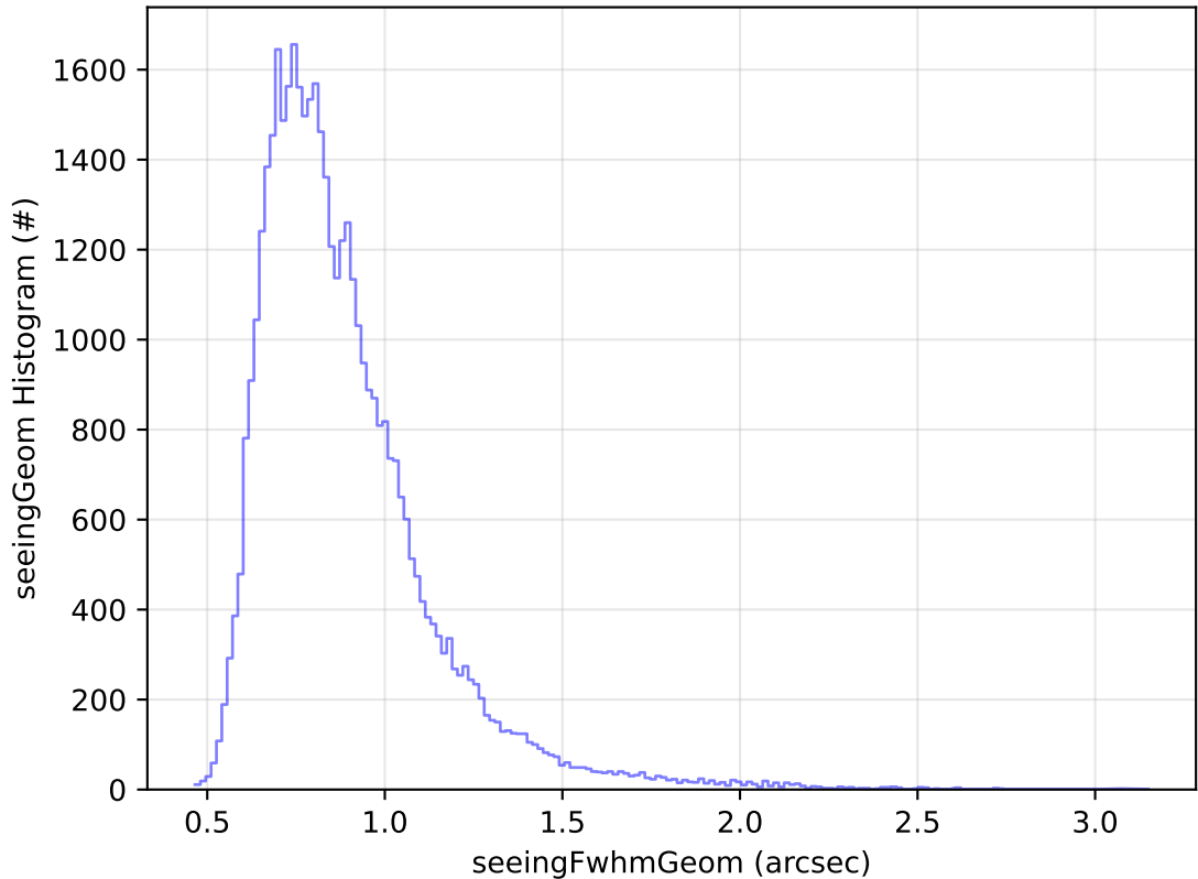
too_combined_no_nss_s10.0_v3.4_10yrs Yr 1 z band: seeingGeom Histogram
