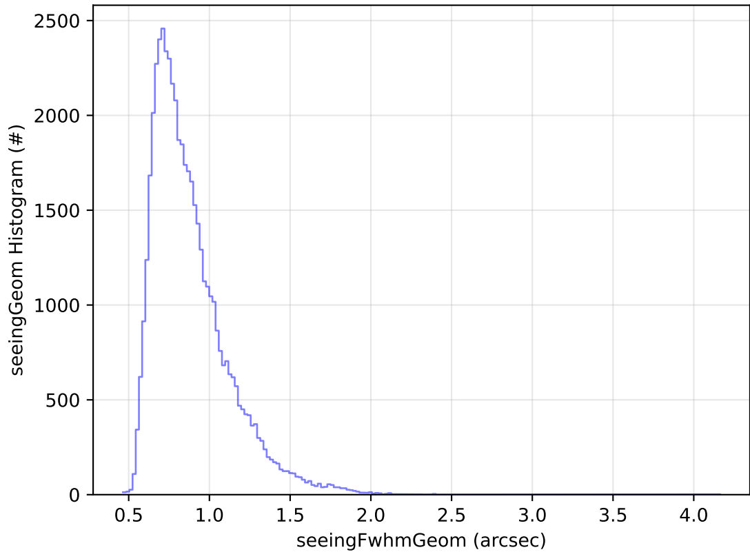
too_combined_no_nss_s10.0_v3.4_10yrs Yr 1 r band: seeingGeom Histogram
