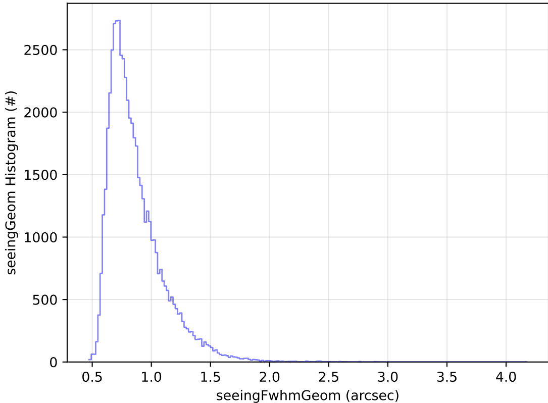
too_combined_no_nss_s10.0_v3.4_10yrs Yr 1 i band: seeingGeom Histogram
