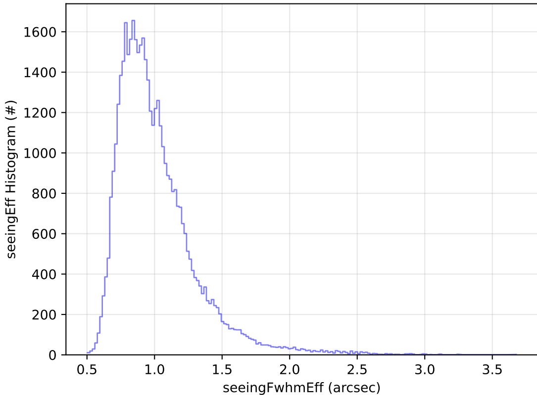
too_combined_no_nss_s10.0_v3.4_10yrs Yr 1 z band: seeingEff Histogram
