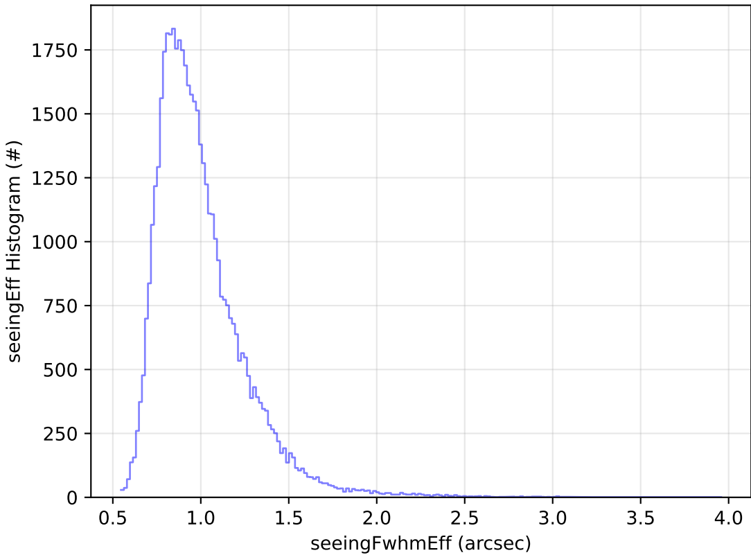
too_combined_no_nss_s10.0_v3.4_10yrs Yr 1 y band: seeingEff Histogram
