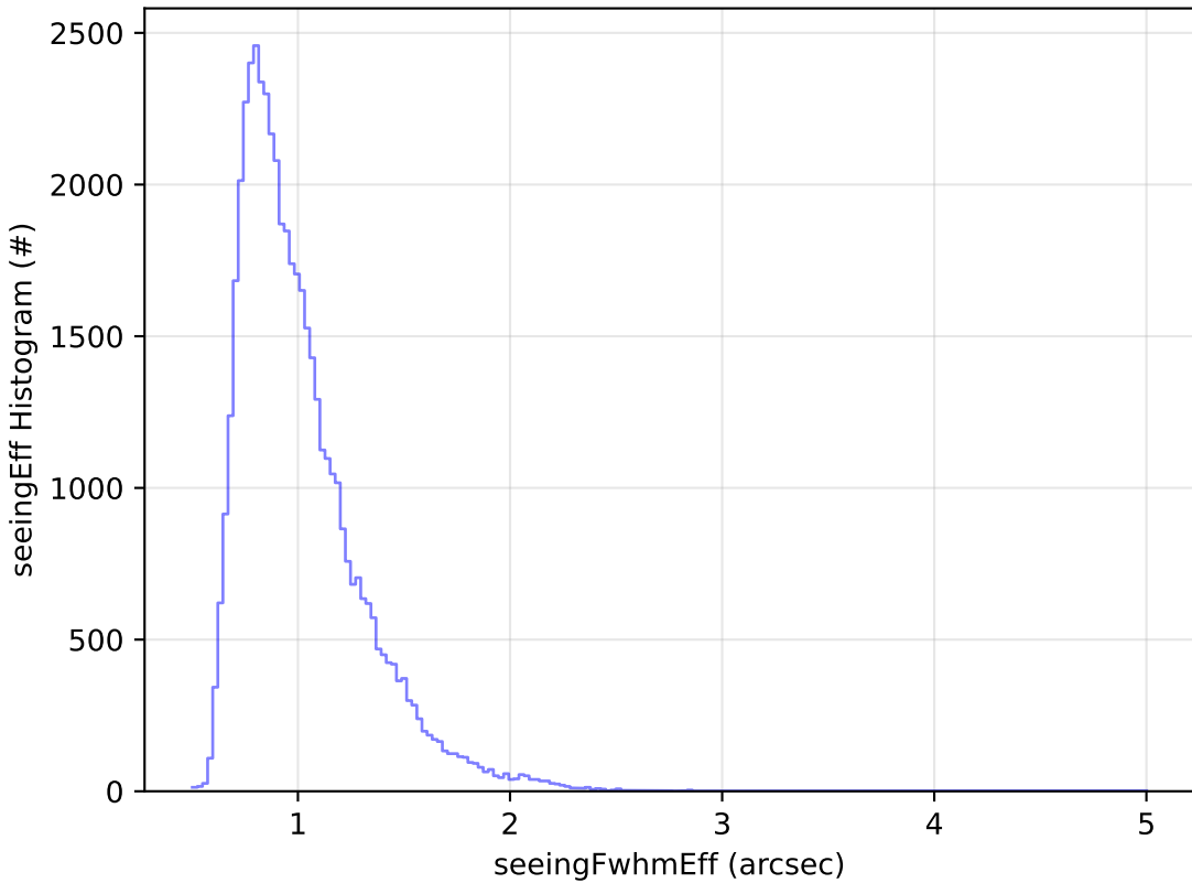
too_combined_no_nss_s10.0_v3.4_10yrs Yr 1 r band: seeingEff Histogram
