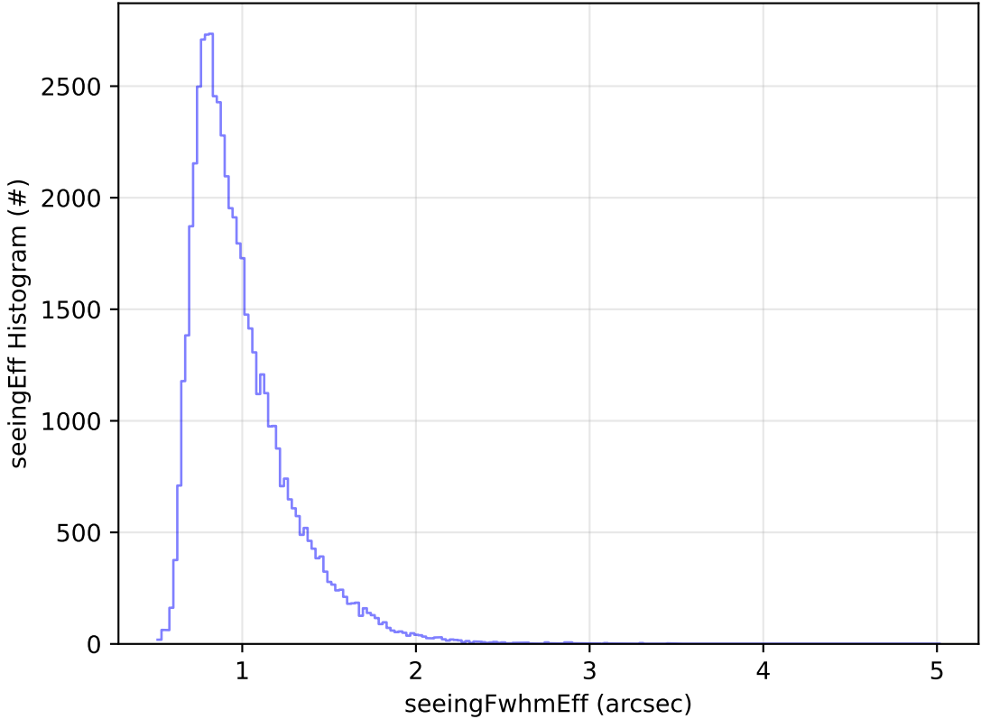
too_combined_no_nss_s10.0_v3.4_10yrs Yr 1 i band: seeingEff Histogram
