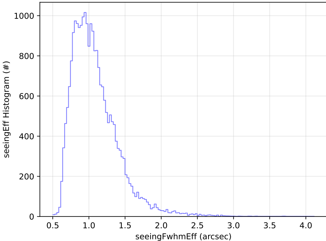
too_combined_no_nss_s10.0_v3.4_10yrs Yr 1 g band: seeingEff Histogram
