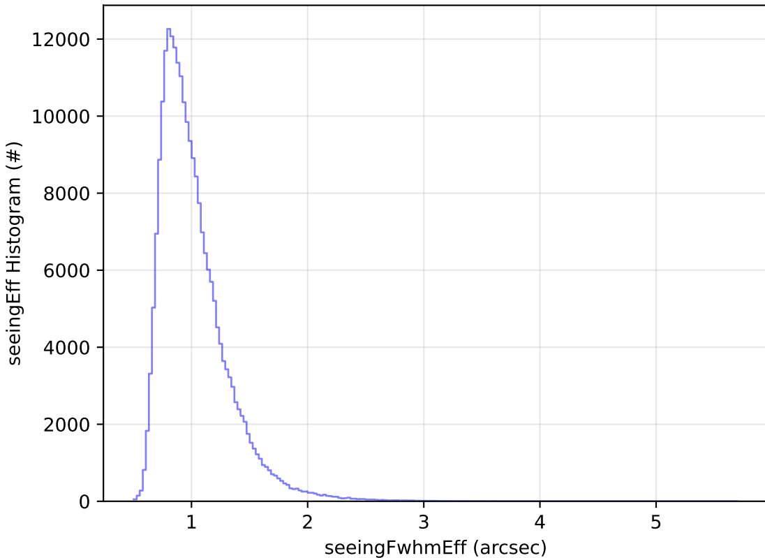
too_combined_no_nss_s10.0_v3.4_10yrs Yr 1 all bands: seeingEff Histogram
