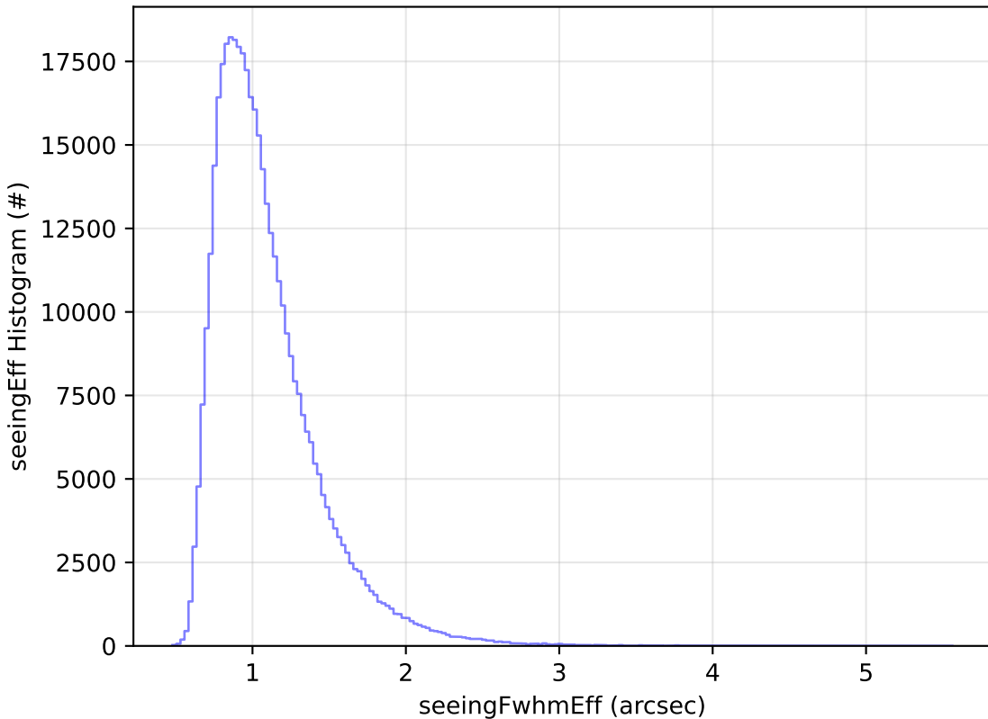
too_combined_no_nss_s10.0_v3.4_10yrs WFD z band: seeingEff Histogram
