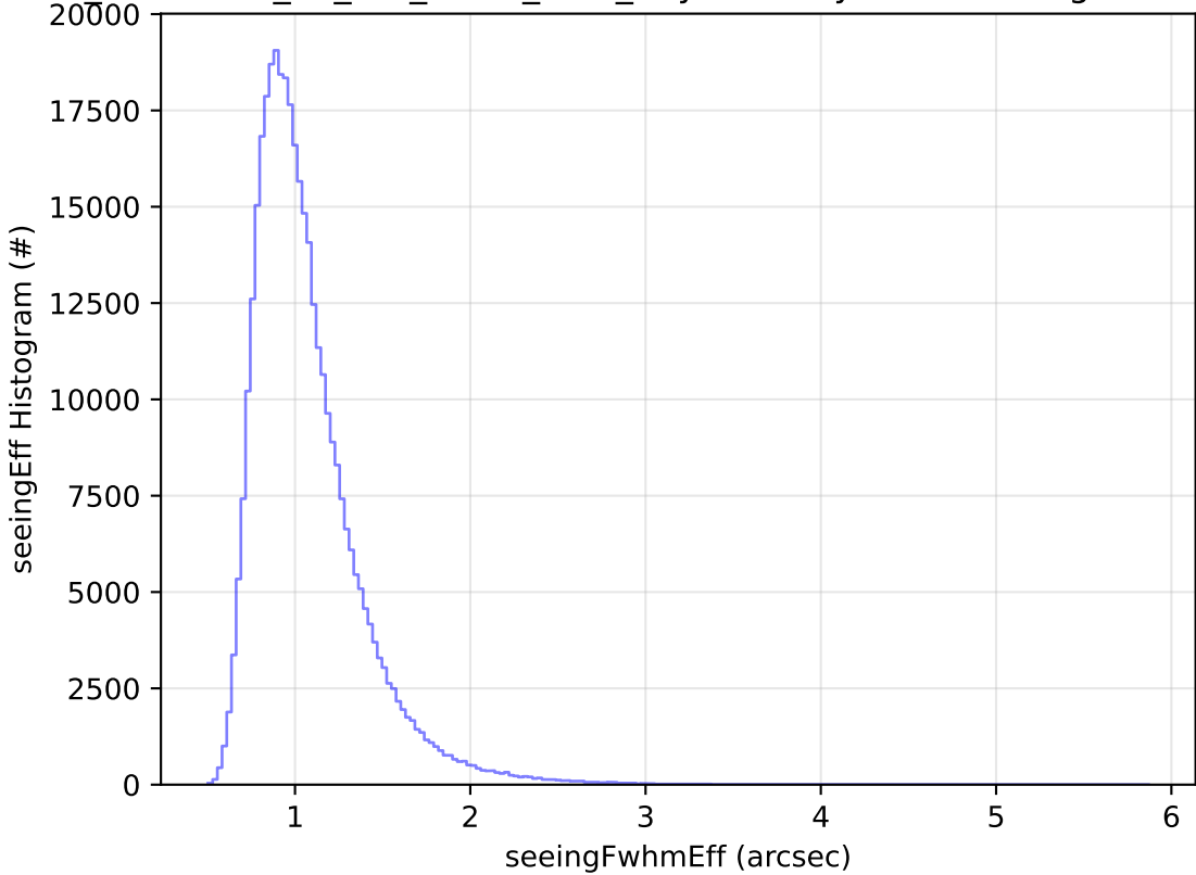
too_combined_no_nss_s10.0_v3.4_10yrs WFD y band: seeingEff Histogram
