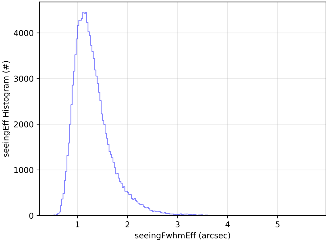
too_combined_no_nss_s10.0_v3.4_10yrs WFD u band: seeingEff Histogram
