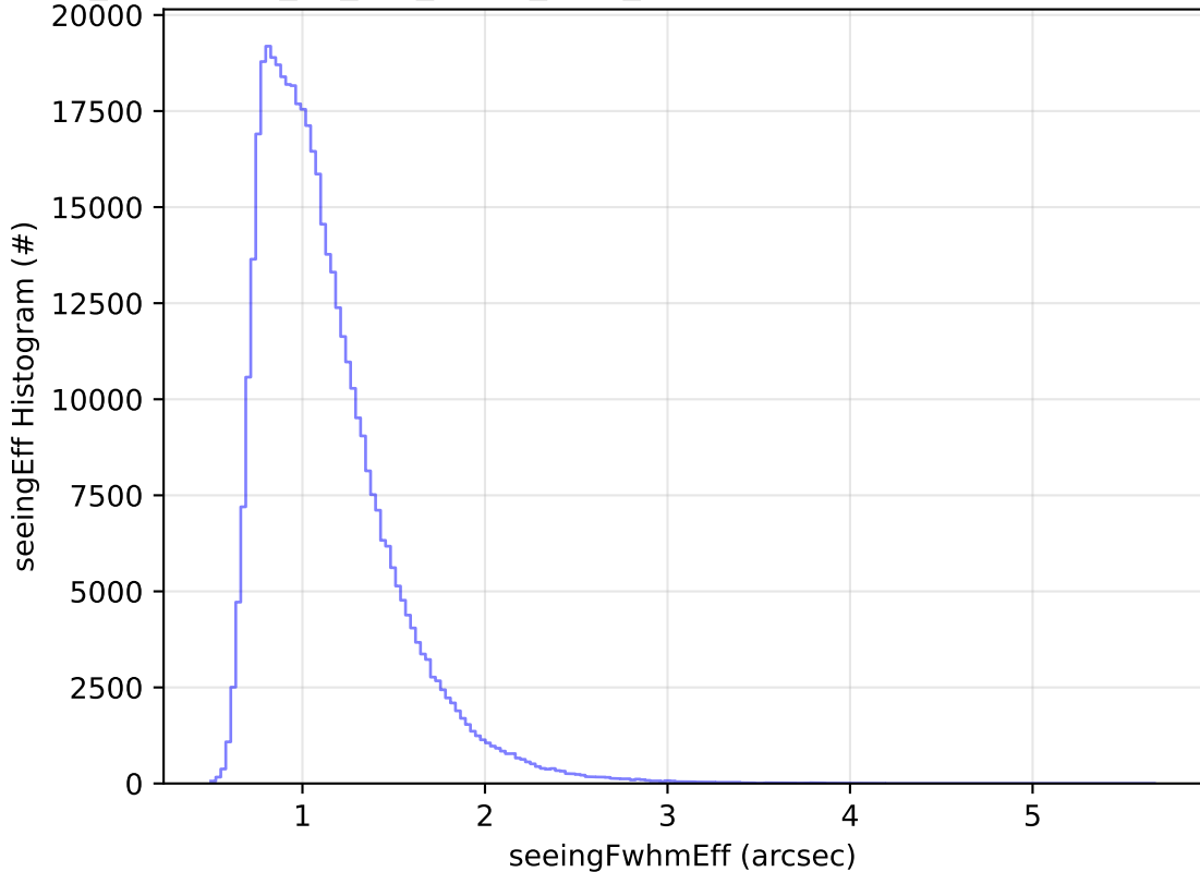
too_combined_no_nss_s10.0_v3.4_10yrs WFD r band: seeingEff Histogram
